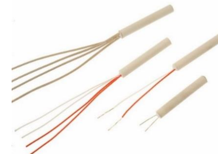
C Pt100 Tubular Ceramic Insert Elements with tail wires
